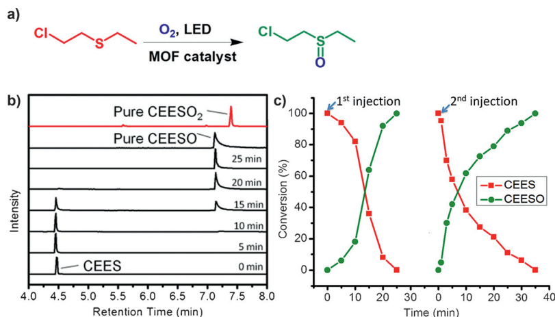
Figure 2. a) Photooxidation of CEES under LED irradiation and O 2 atmosphere catalyzed by MOF-based catalyst fb-1. b) Gas chromatography (GC) signals indicating the progress of the oxidation of CEES (4.45 min) to CEESO (7.14 min) in the presence of fb-1 (1.2 mg). For comparison, chromatograms of pure CEESO (7.14 min) and pure CEESO 2 (7.38 min) were also recorded, confirming that CEESO was the only product. c) Oxidation profile of CEES in the presence of fb-1 (1.2 mg) while being irradiated with a blue LED with two consecutive injections of CEES (0.2 mmol).
